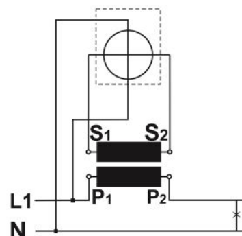
Energy Meter multiple phases
